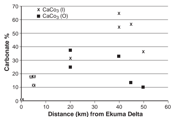
Fig. 5: Carbonate content of the inner and outer dune along transects from the delta. (I) – inner dune, (O) – outer dune.
