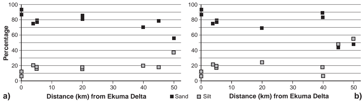
Fig. 4: Sand and silt grain composition along transects from the Ekuma delta. (a), outer dune, and (b), inner dune.
