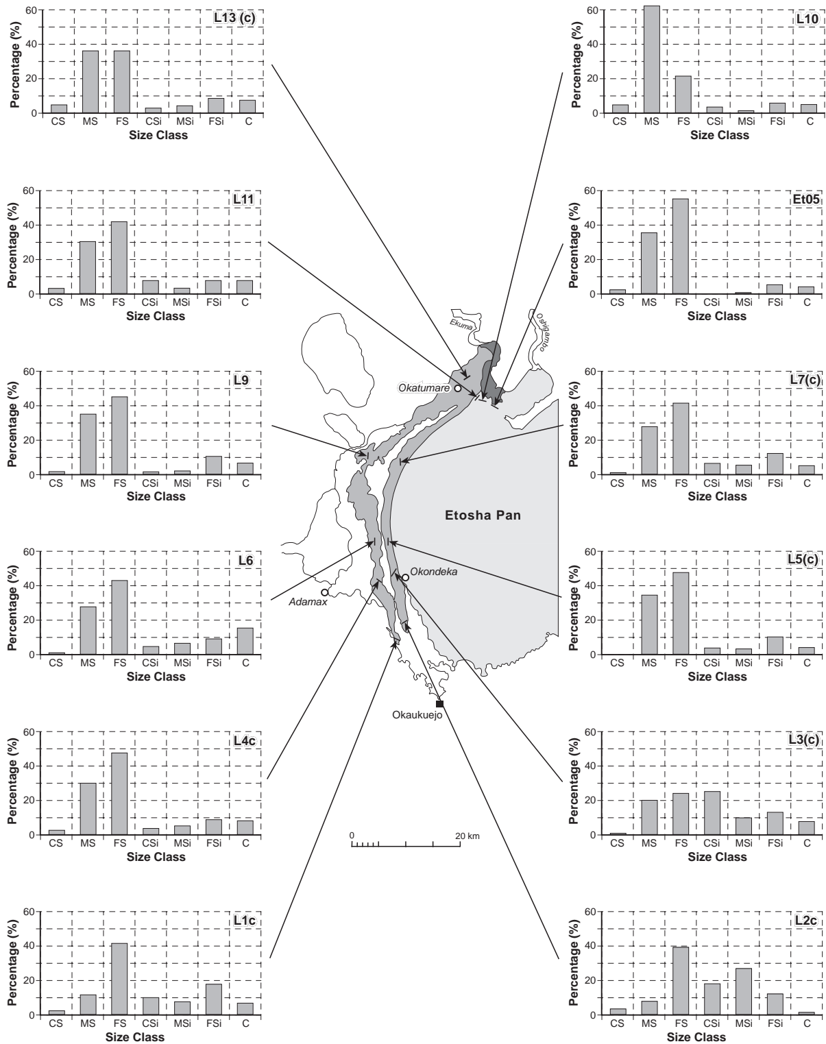
Fig 3: Selected ratios of sand, silt, and clay along the dunes and at the Ekuma delta. Key: CS – coarse sand, MS – medium sand, FS – fine sand, CSi – coarse silt, MSi – medium silt, FSi – fine silt, C – clay.
